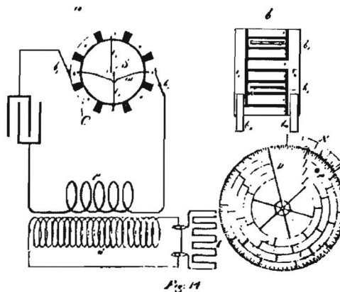
Figure 92 (above). Illustrating some of the attachments and mode of using same. Houston Street Laboratory, 1898-1900.
