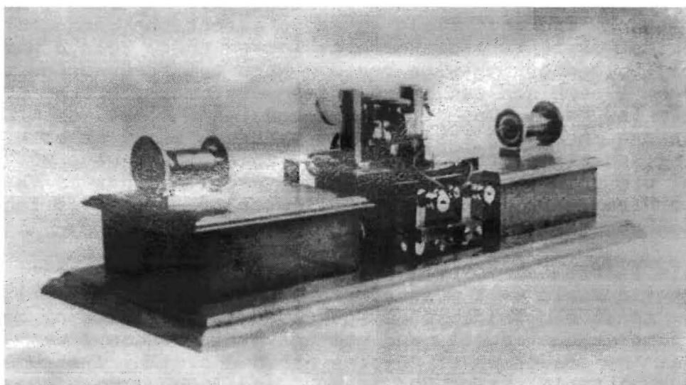
Figure 13. Instrument to receive radio waves of 1896-1899 structure.
