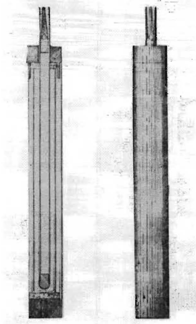
Figure 16. Improved form of electrolyte condenser as used in laboratories on 35 S. Fifth Avenue and 46 E. Houston Street.
