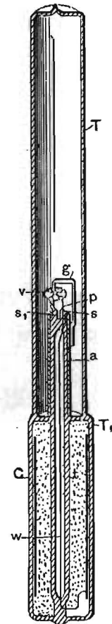
Figure 63. Striking experiment in the transmission of energy by electromagnetic waves. Demonstrated in lectures before the Institution of Electrical Engineers and the Royal Institution, London, in February 1892. Illustrated in Martin book, Fig. 164, p. 288.
