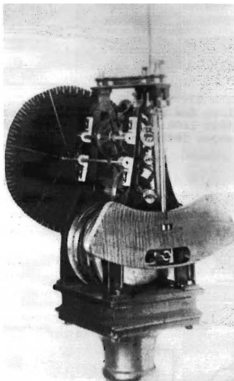
Figure 91 (left). Special clock constructed for purpose of measurements, especially useful in receiving. Described in lecture before The New York Academy of Sciences, 1897.
