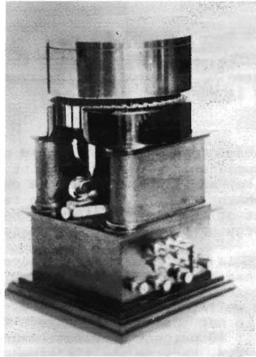
Figure 44. One of the many forms of mercury circuit controllers described in various U.S. Patents.
