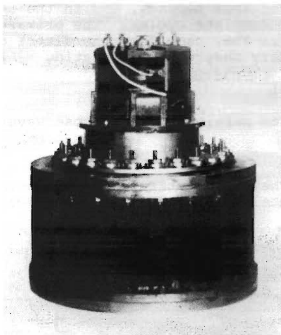
Figure 47. Large mercury circuit controller of high frequency (telegraphic and telephonic experiments).
