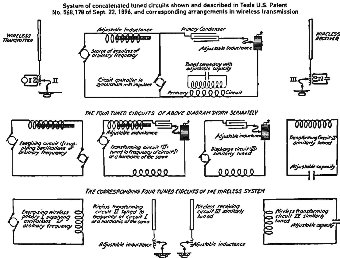
Figure 66. Diagrams illustrating the system of four-tuned circuits as applied to wireless transmission. Described in U.S. Patent No. 568,178 of September 22, 1896. Application filed June 20, 1896.
